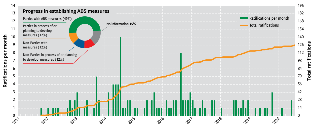
Figure 16.1. Trends in the ratification of the Nagoya Protocol and in the progress of establishing ABS measures
