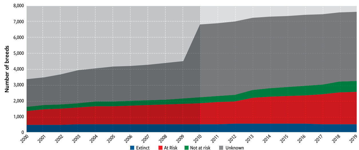
Figure 13.2. Trends in status of local breeds according to risk categories.
