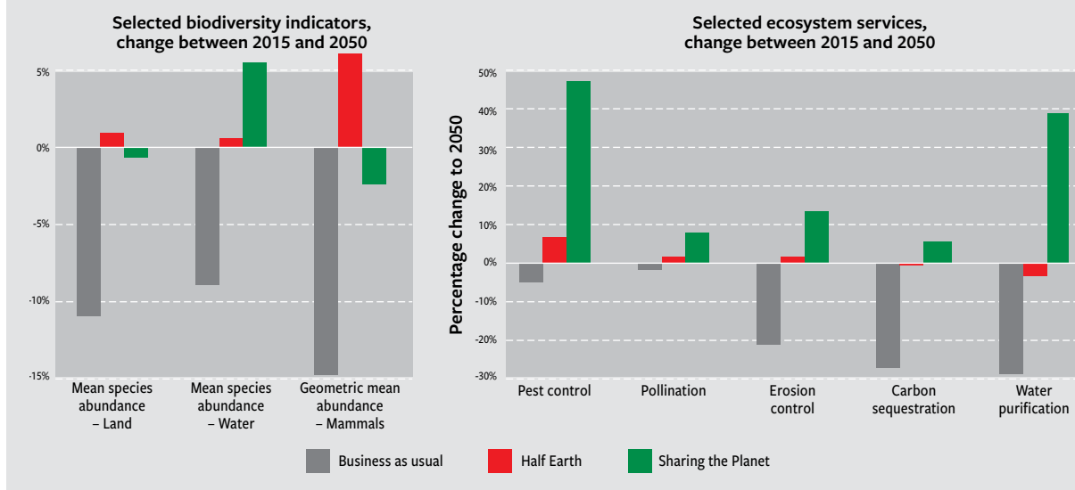
Figure 22.2. Outcomes in projected change to biodiversity and ecosystem services between 2015 and 2050, for ‘business as usual’, ‘Half Earth’ and ‘Sharing the Planet’ scenarios, including additional measures for climate change mitigation and sustainable consumption. 18
