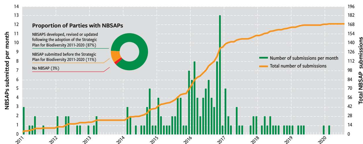
Figure 17.1. Extent and timing of submission of national biodiversity strategies and action plans 2
